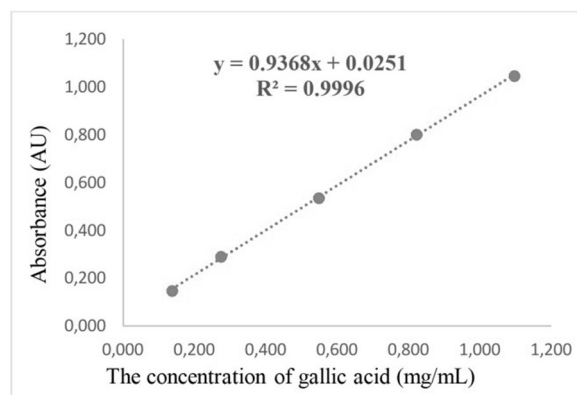
Fig. 1. Calibration curves for gallic acid
